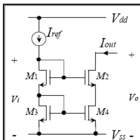
مدار ۱ (current mirror1.sp)
