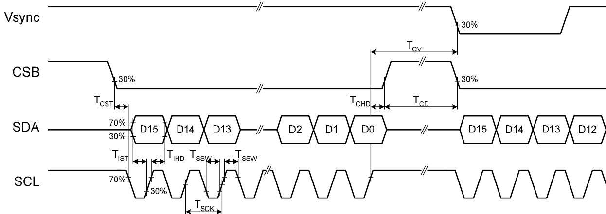
Figure 6 : AC serial interface write mode timing
