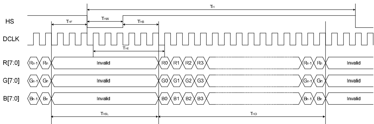
Figure 2 Horizontal input timing. (HV mode)
