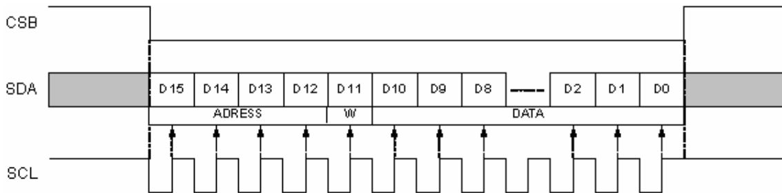
Figure 7: Serial interface write sequence
