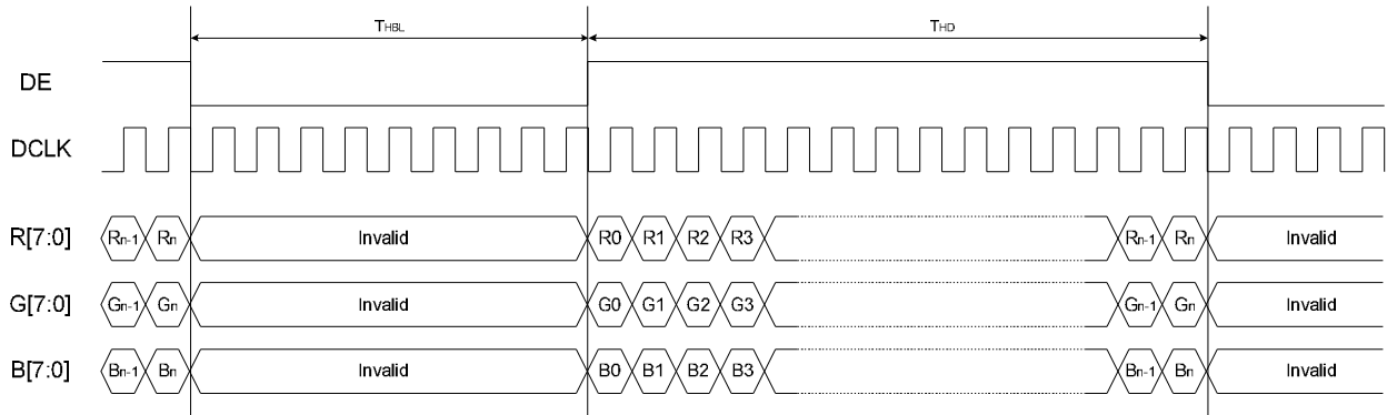
Figure 3: Horizontal input timing. (DE mode)
