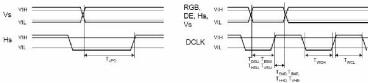
Figure 1 : Input timing details
