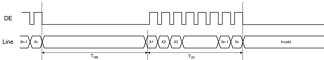
Figure 5: Vertical timing. (DE mode)
