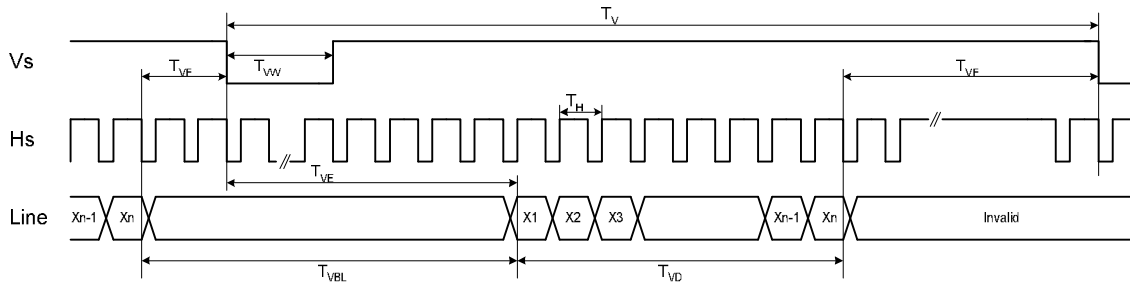
Figure 4: Vertical timing. (HV mode)
