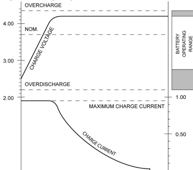
Figure 1-1. Charge stages and limits of a Varta PoLiFlex® cell
